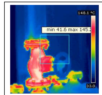
BELLOW SEAL GLOBE VALVE
