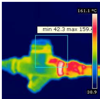
THERMODYNAMIC STEAM TRAP
